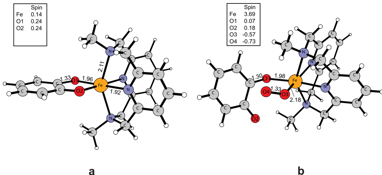
Figure 3: a) The reactant R1 in its ground state, b) the superoxide complex R2 .
