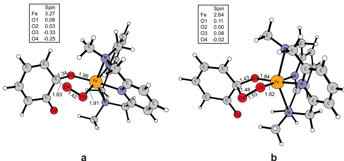
Figure 5: a) Transition state for peroxide formation TS1 , b) the bridging peroxide BP
