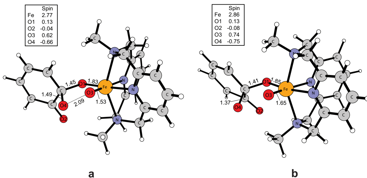
Figure 6: a) Transition state for the homolytic O-O bond cleavage {}^4\text{TS2} , b) the alkoxy radical, RAD , formed after the O-O bond cleavage.
