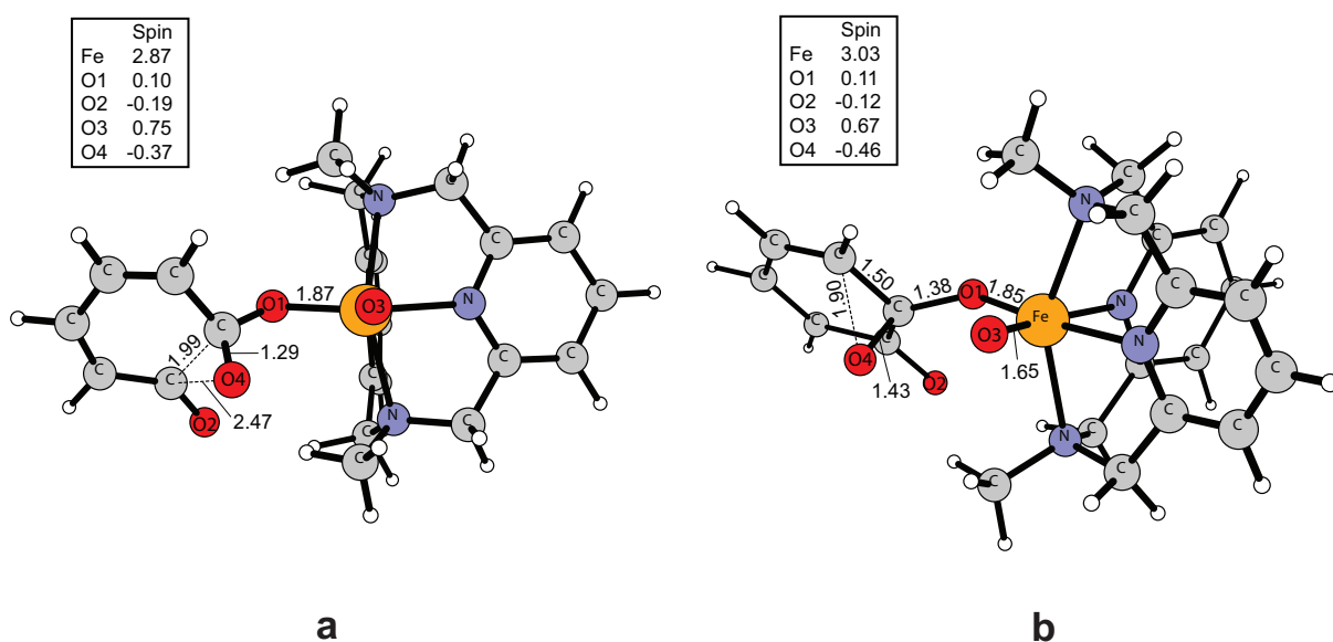
Figure 8: a) Transition state for intradiol cleavage {}^4\text{TSi} , b) Transition state for epoxide formation {}^4\text{TSe}
