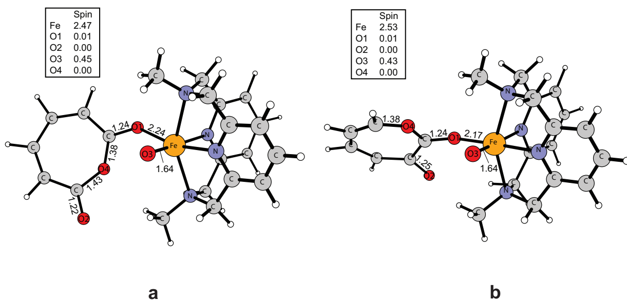
Figure 9: a) The anhydride product of the intradiol cleavage ANH , b) the lactate product of the extradiol pathway LA .
