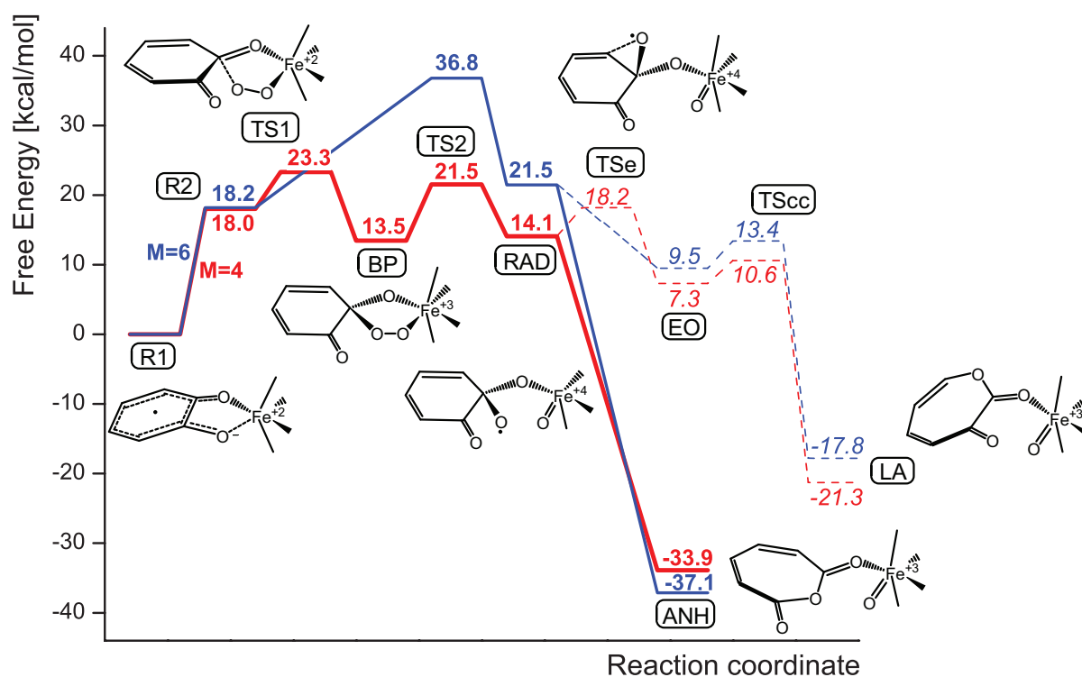
Figure 7: Calculated energy profile along the reaction coordinate; red - quartet state PES, blue - sextet state PES, solid line - the observed intradiol reaction path, dashed line - the alternative extradiol reaction path.
