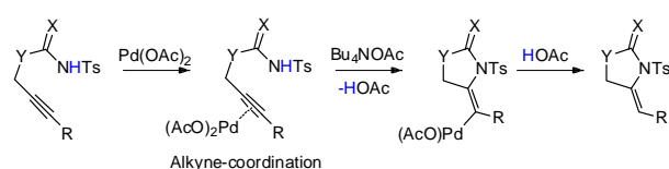
Scheme 2. Plausible palladium-catalyzed cyclization mechanism.
