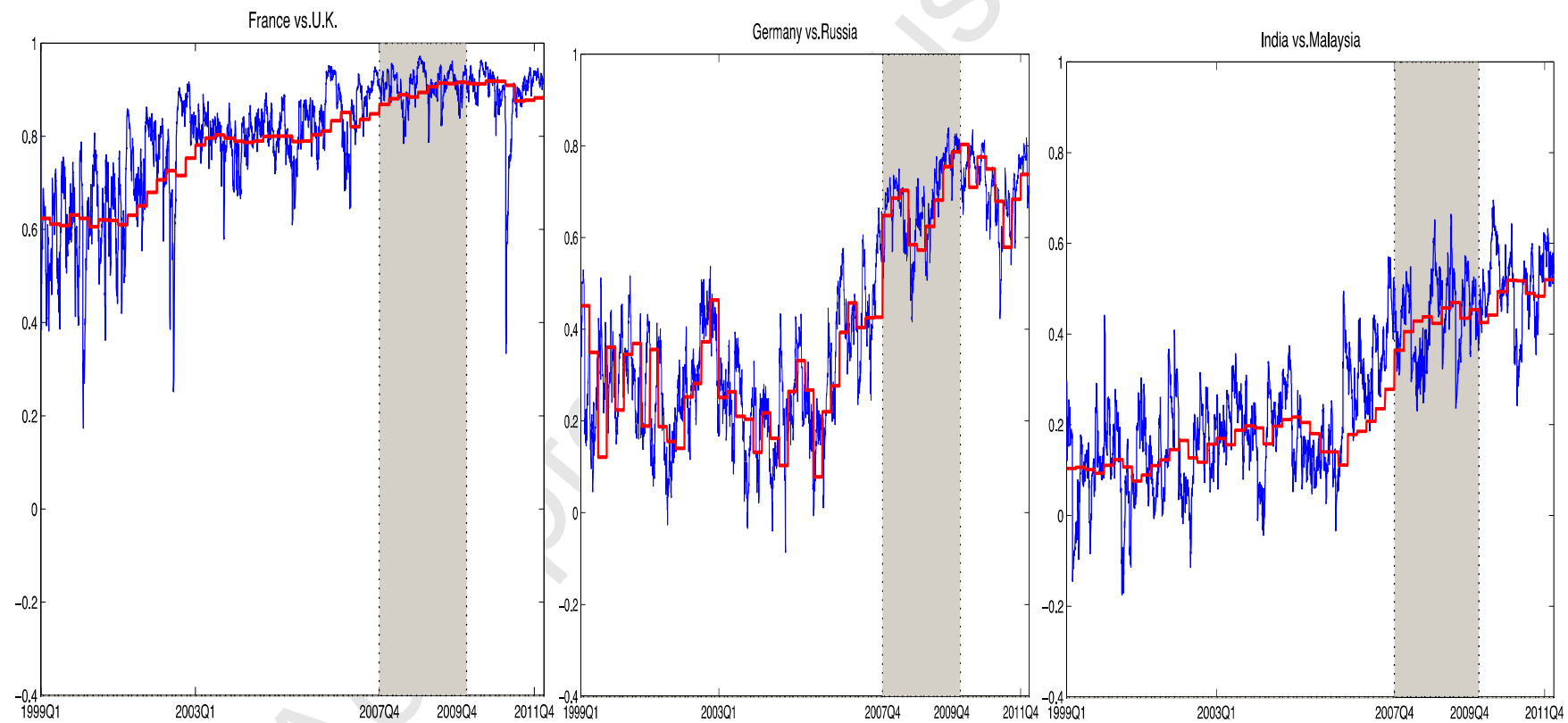
Figure 1.2: The short and long DCC MIDAS correlations for chosen countries
